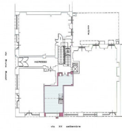
PIANO TERRENO
