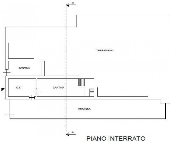
PIANO INTERRATO
